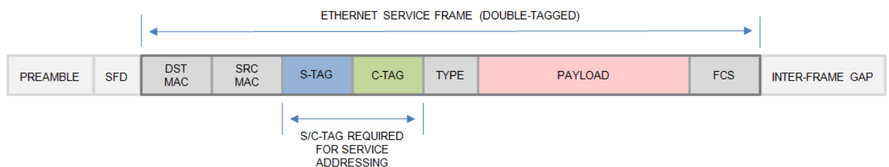
Figure 4 Service Addressing Mode A Frame Format 4
