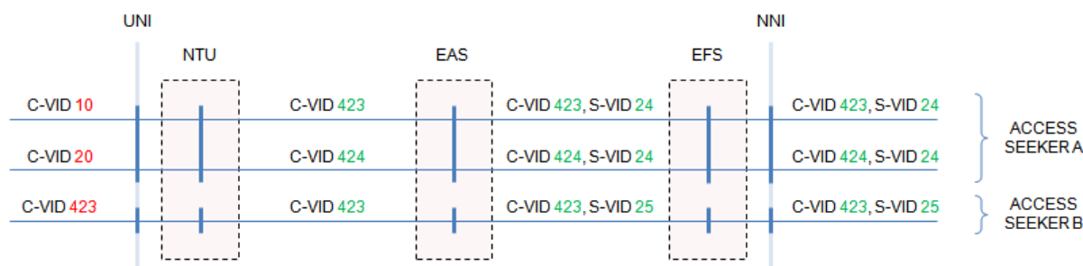
Figure 20 Example Tagged UNI-D
